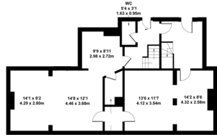
GROUND FLOOR (24)
